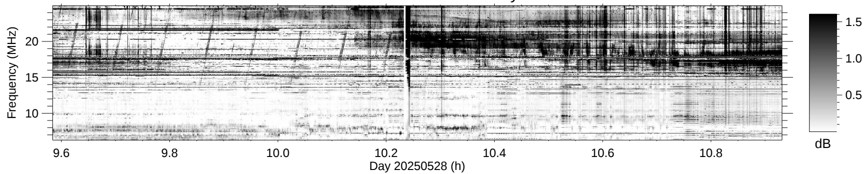
NDA/JunoN LH flux density
