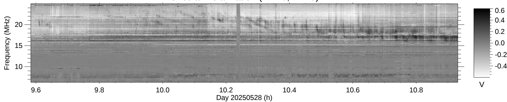
Circular Polarization (RH<0, LH>0)
