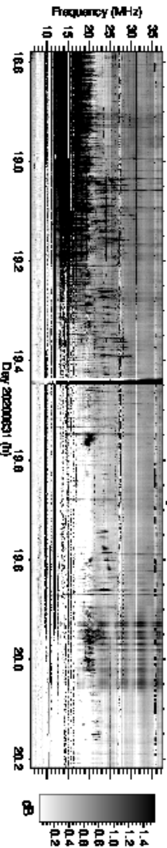
NDA/Juno RH flux density
