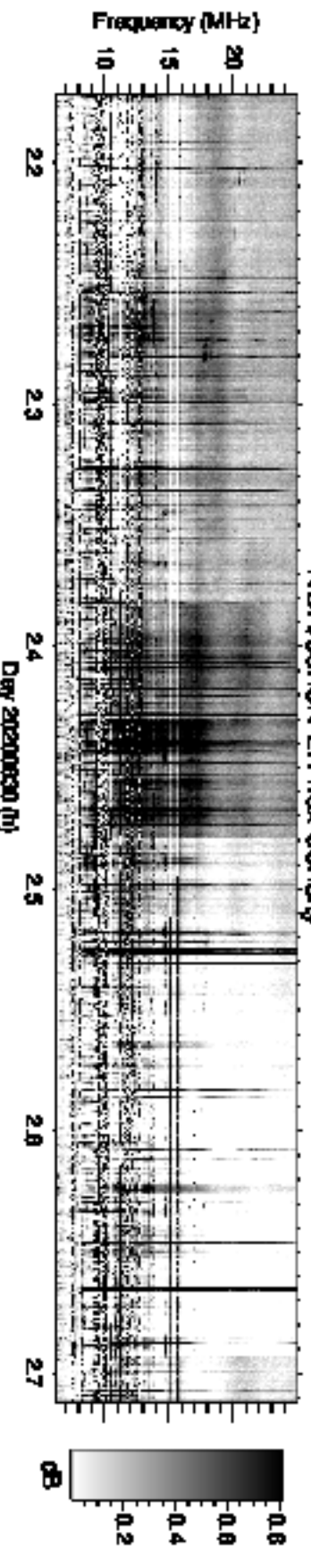
NDA/Jurón LH flux density
